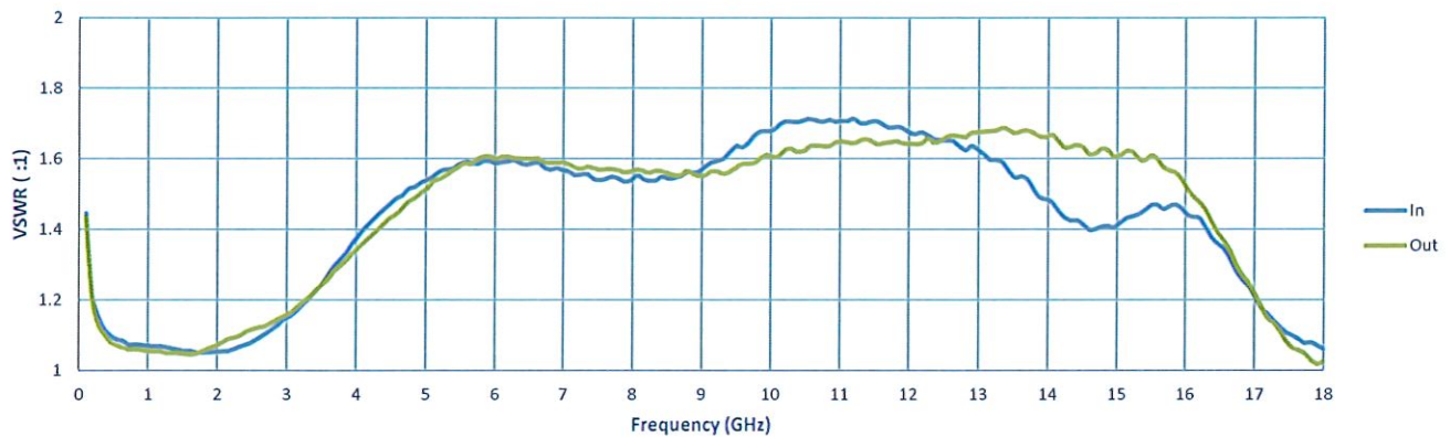
VSWR @ -20 dB
