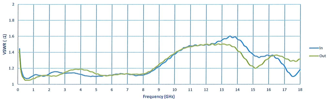
VSWR @ -20 dB
