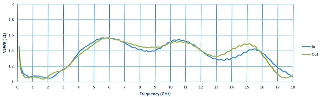
VSWR @ -20 dB
