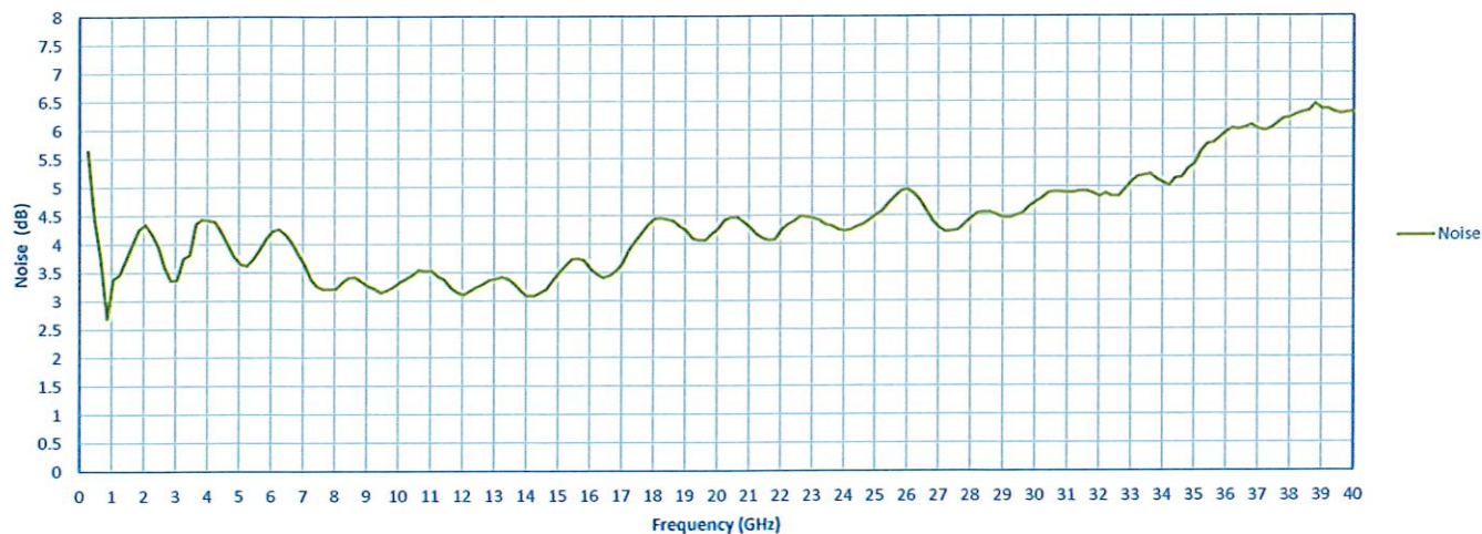
Noise Figure
