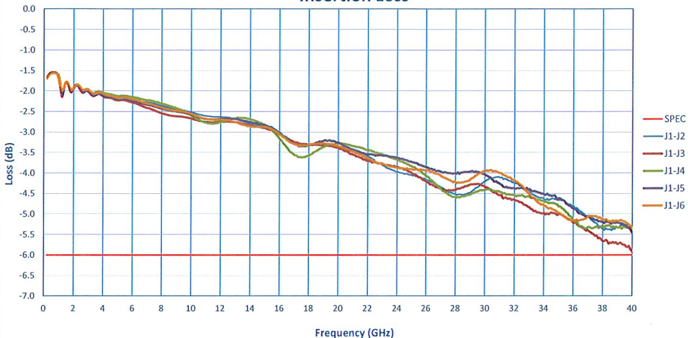
Insertion Loss
