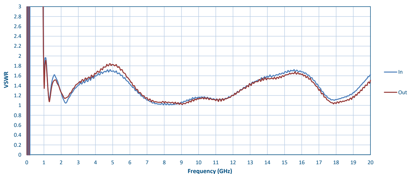
VSWR Passband Vs Frequency
