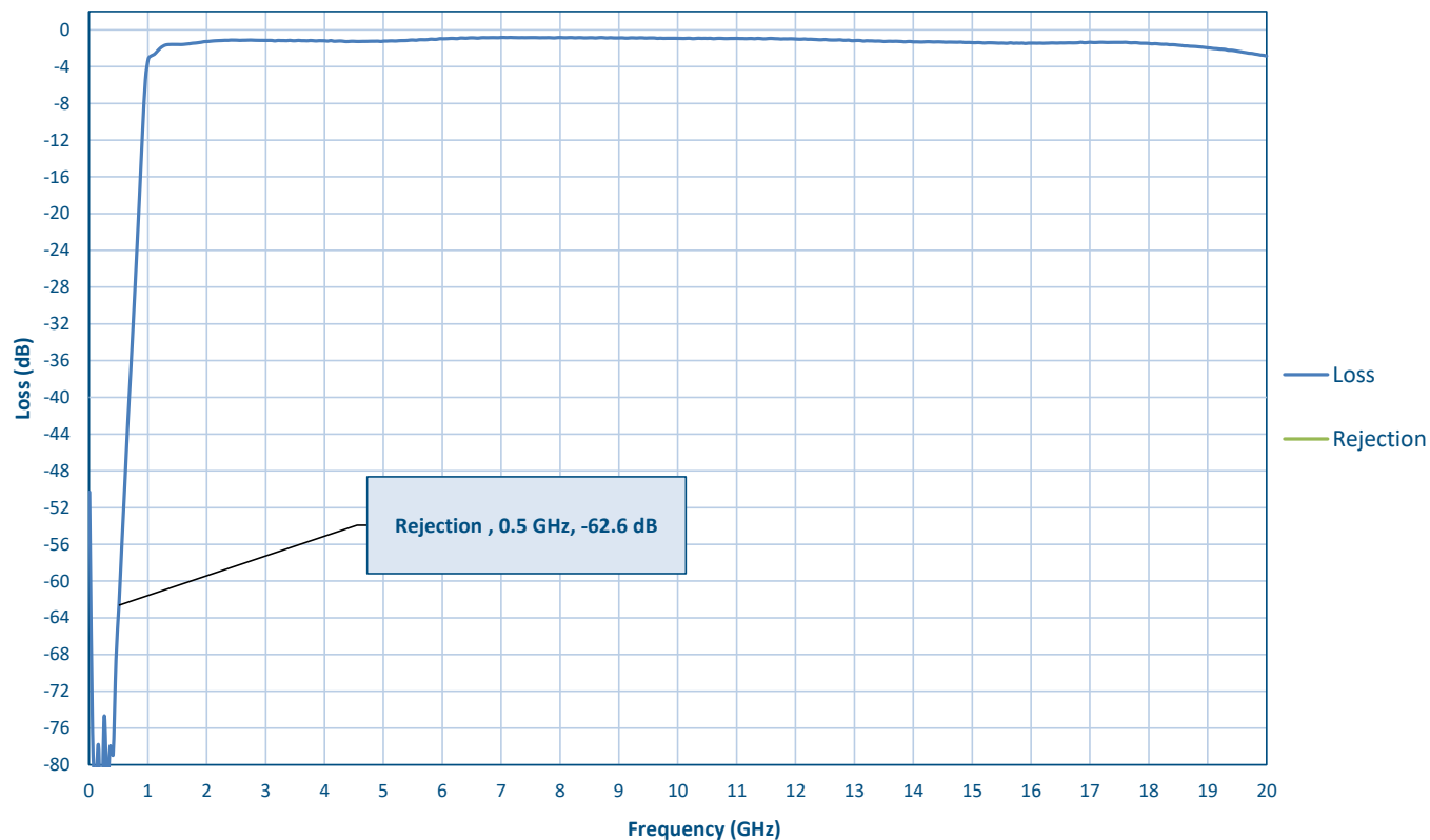
Insertion Loss Passband Vs Frequency
