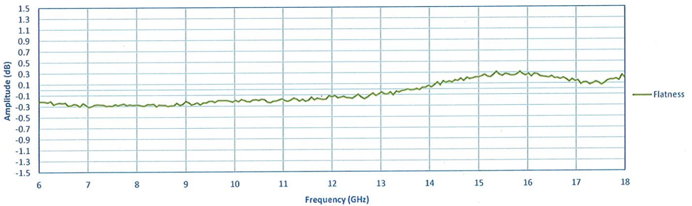
Gain Flatness
