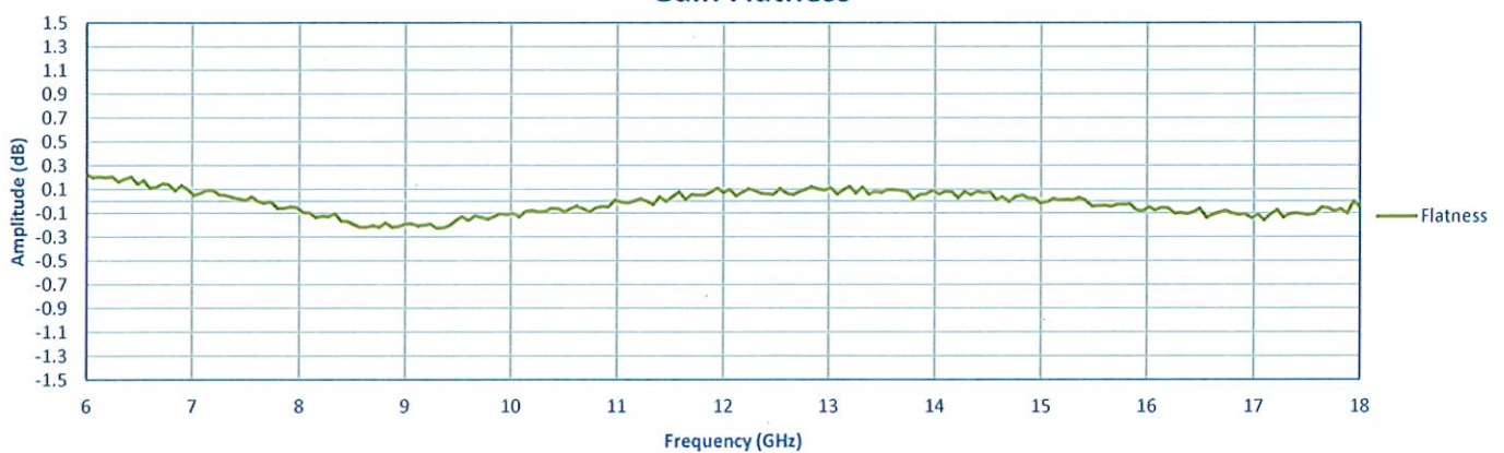
Gain Flatness
