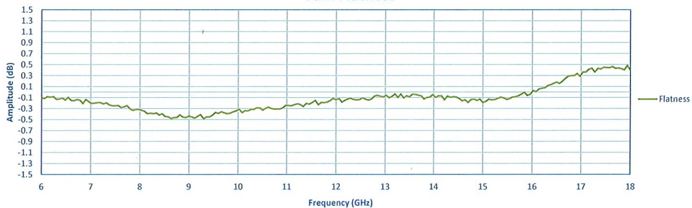
Gain Flatness
