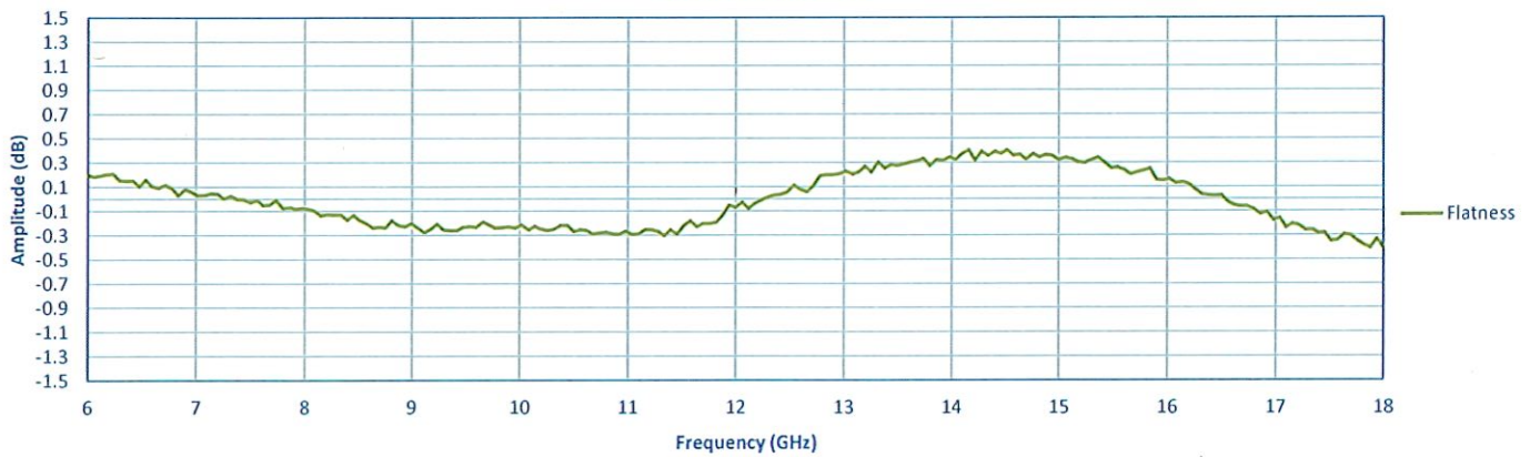
Gain Flatness
