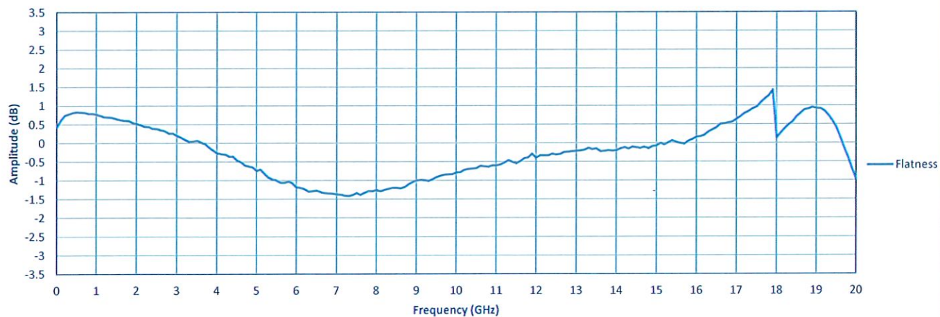
Gain Flatness
