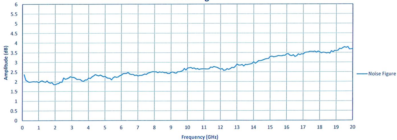
Noise Figure
