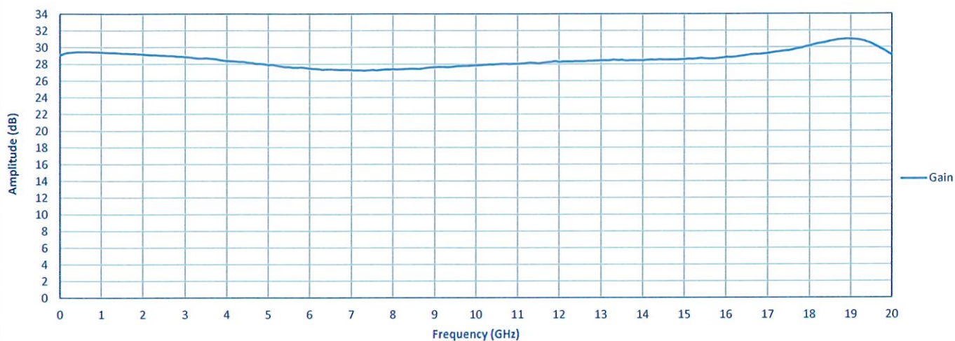
Gain
