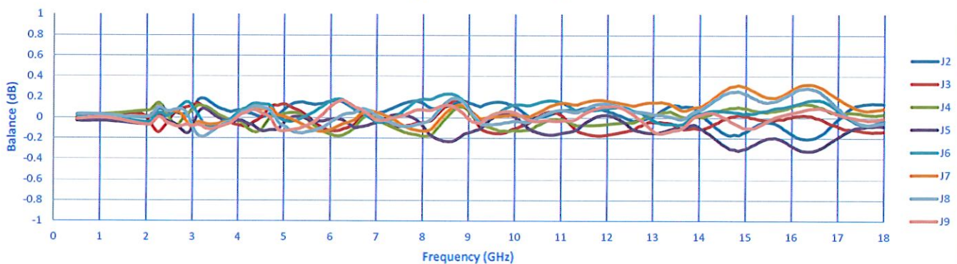
Amplitude Balance
