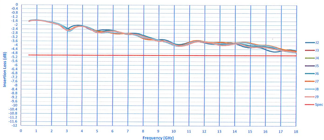
Insertion Loss
