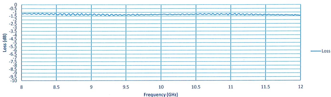
Insertion Loss
