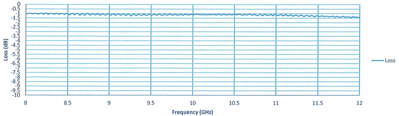
Insertion Loss
