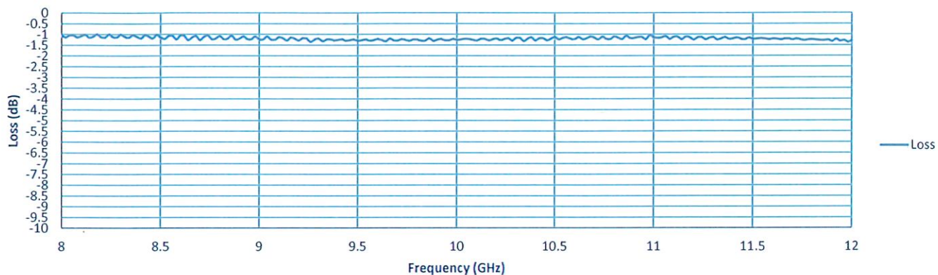
Insertion Loss
