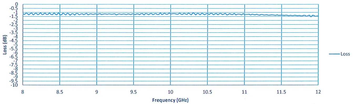
Insertion Loss
