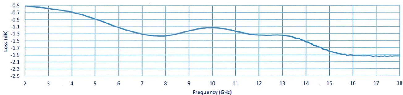
Insertion Loss
