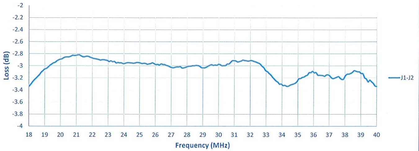
Insertion Loss
