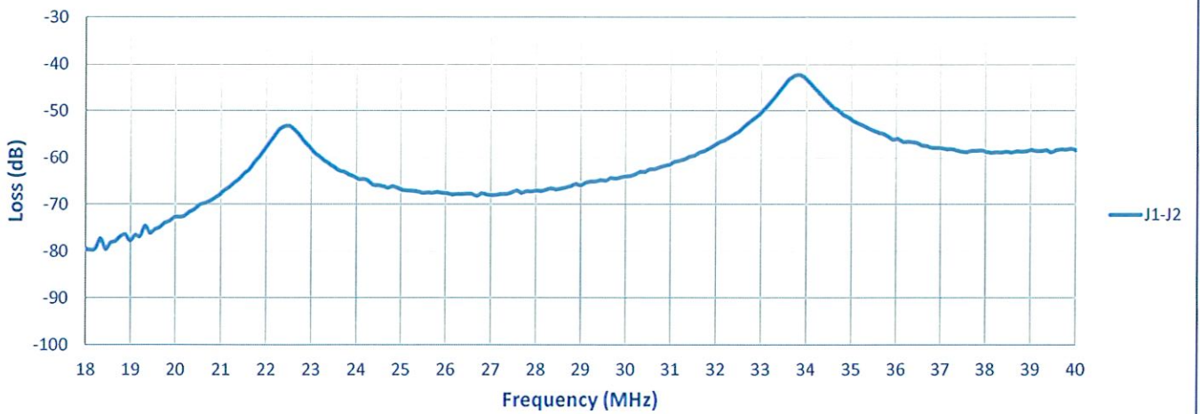
Isolation
