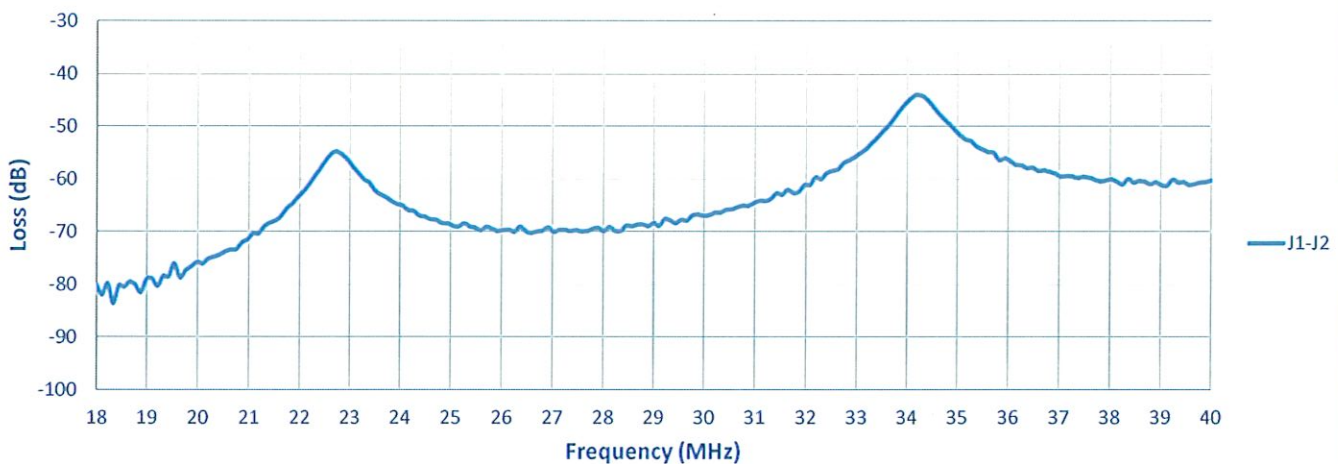
Isolation
