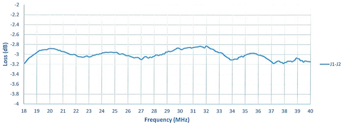
Insertion Loss
