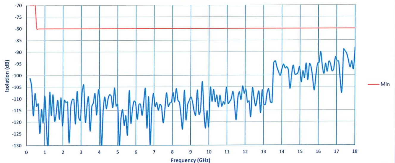
Isolation
