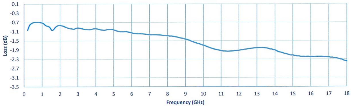
Insertion Loss
