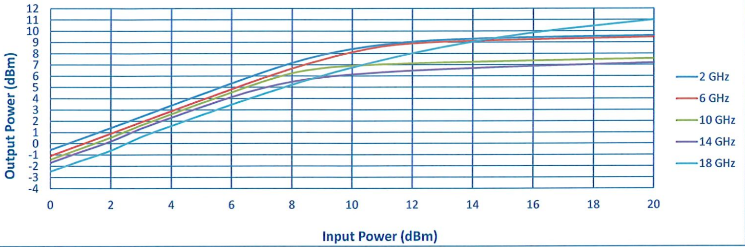
Limiting @ -44°C
