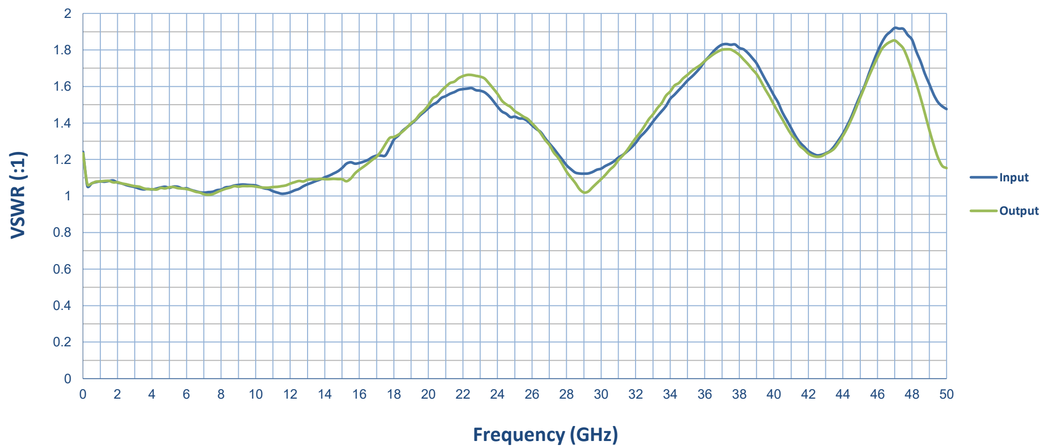
VSWR @ -10 dBm
