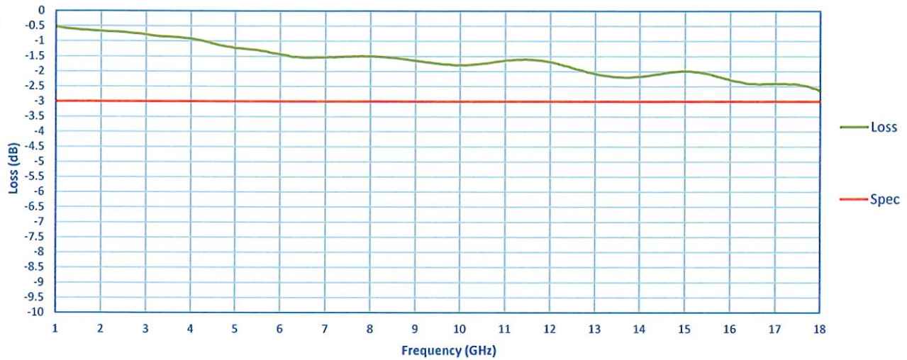
Insertion Loss
