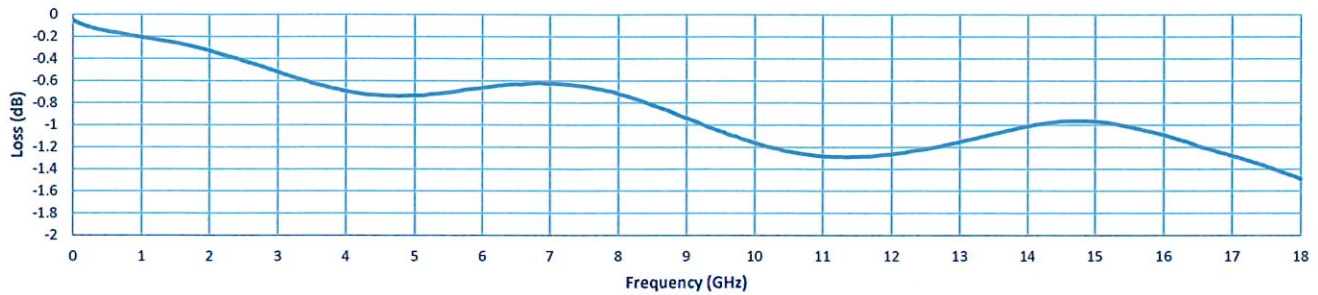
Insertion Loss
