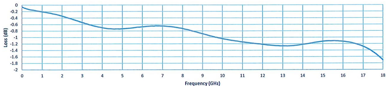
Insertion Loss
