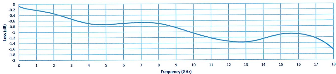
Insertion Loss
