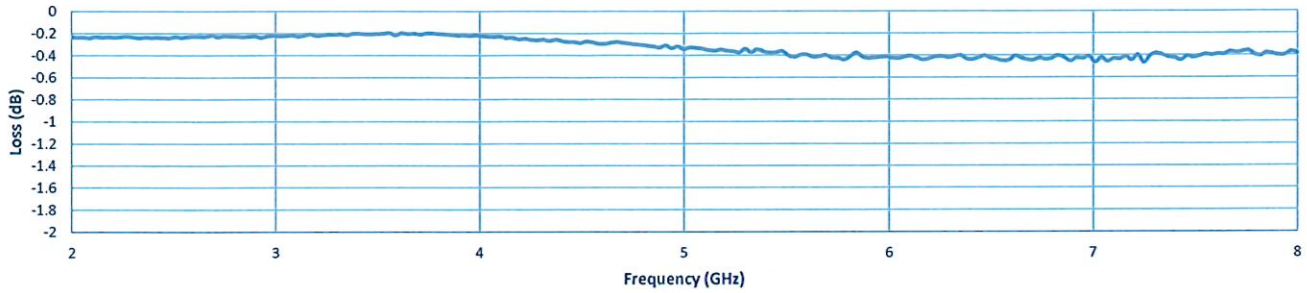
Insertion Loss
