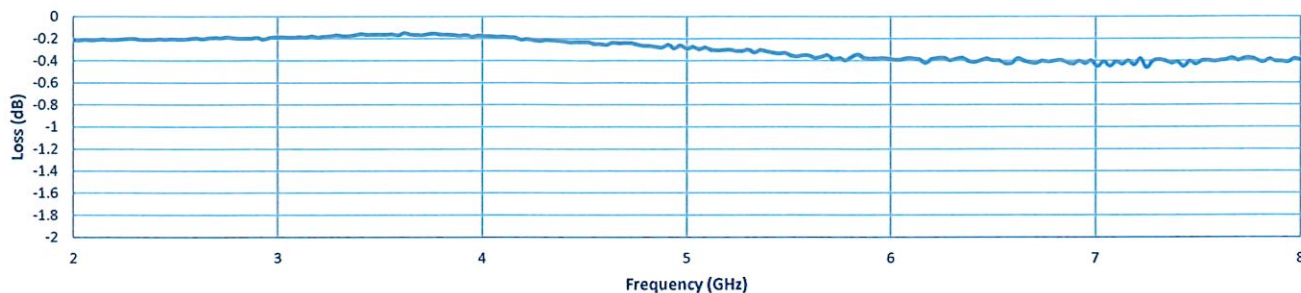
Insertion Loss
