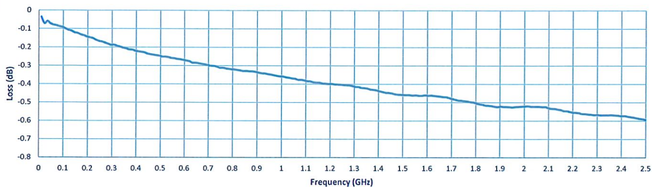
Insertion Loss
