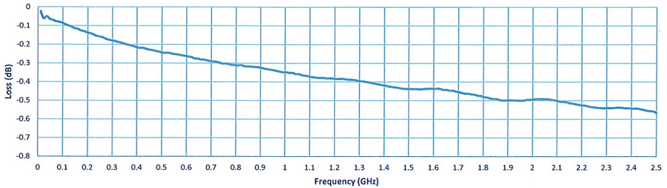
Insertion Loss
