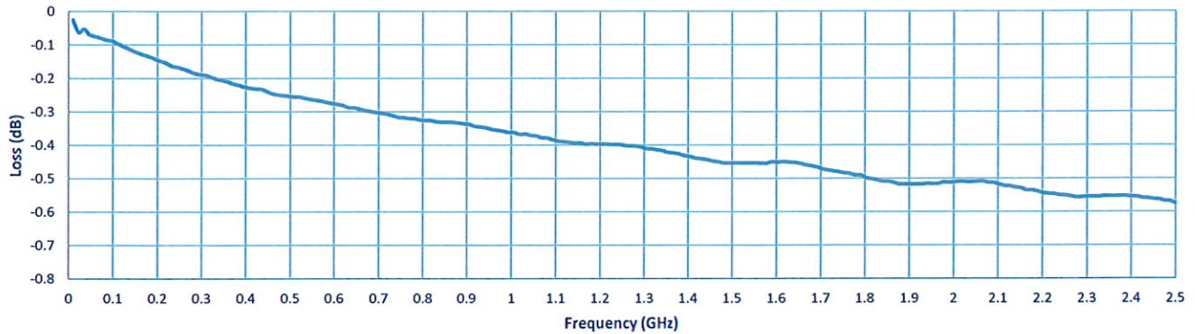
Insertion Loss
