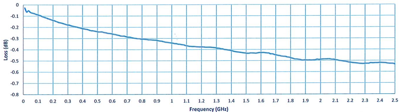
Insertion Loss
