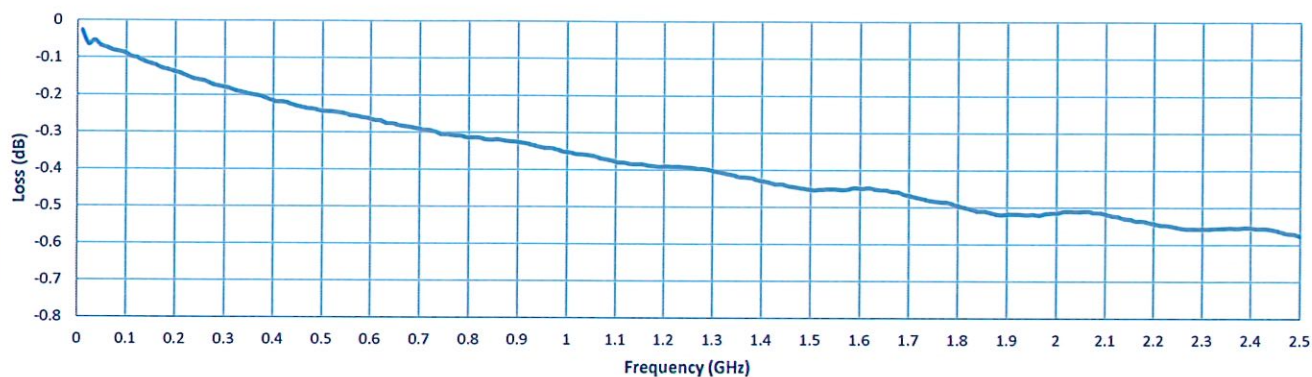
Insertion Loss
