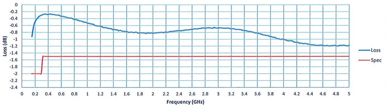
Insertion Loss
