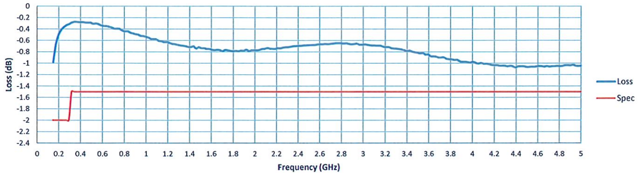
Insertion Loss
