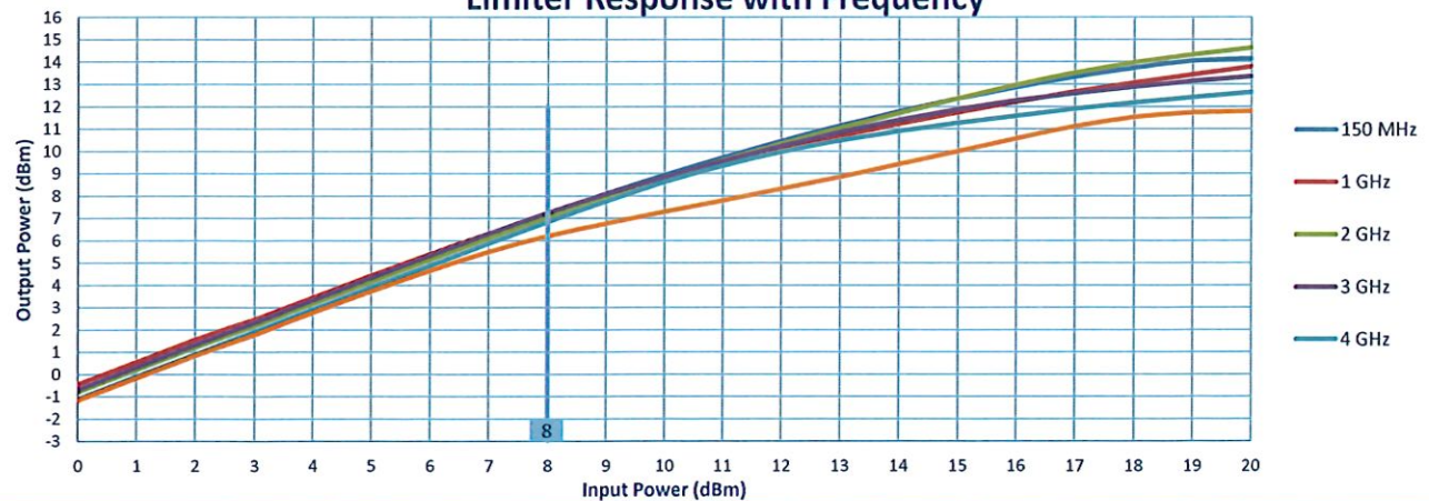
Limiter Response with Frequency
