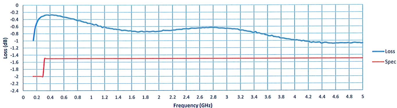
Insertion Loss
