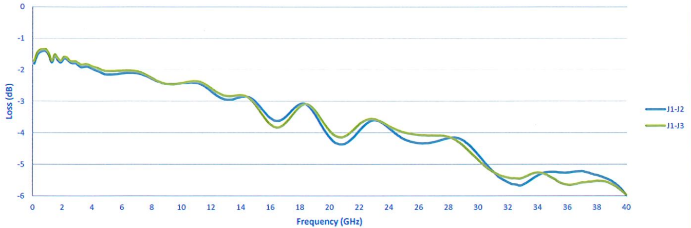
Insertion Loss
