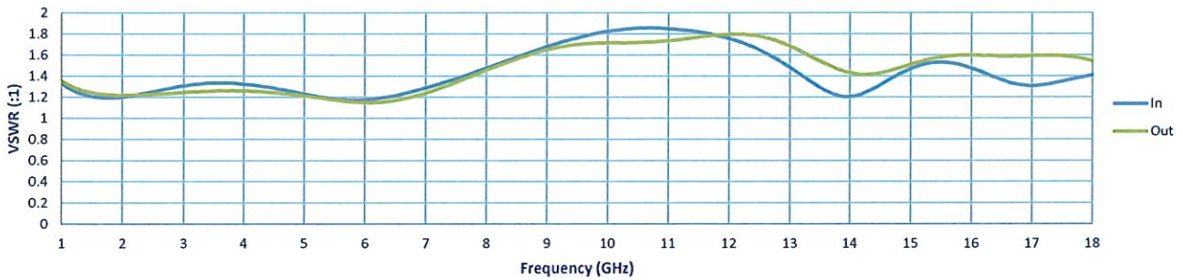
VSWR @ -20dBm
