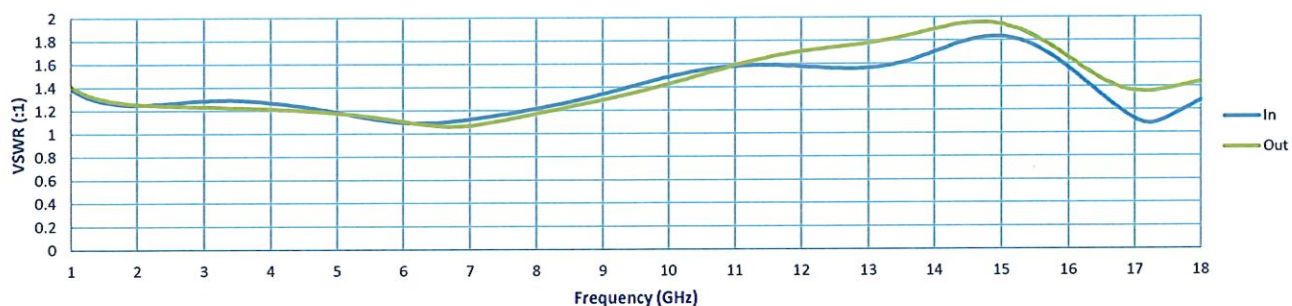
VSWR @ -20dBm
