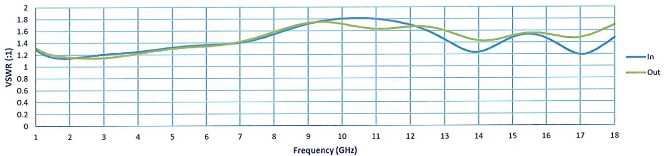
VSWR @ -20dBm
