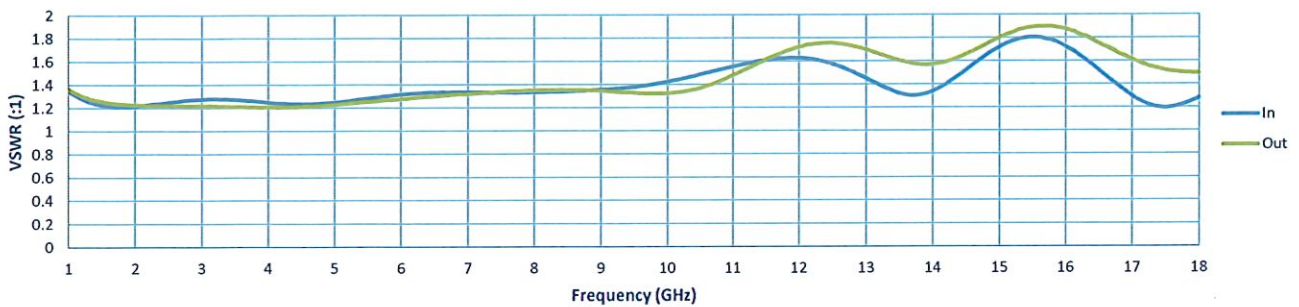
VSWR @ -20dBm
