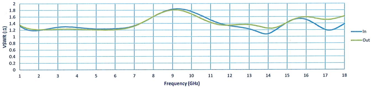
VSWR @ -20dBm
