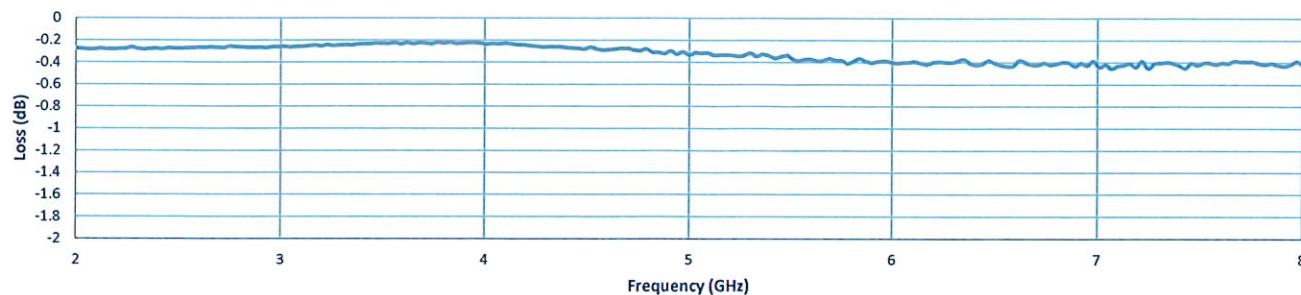
Insertion Loss
