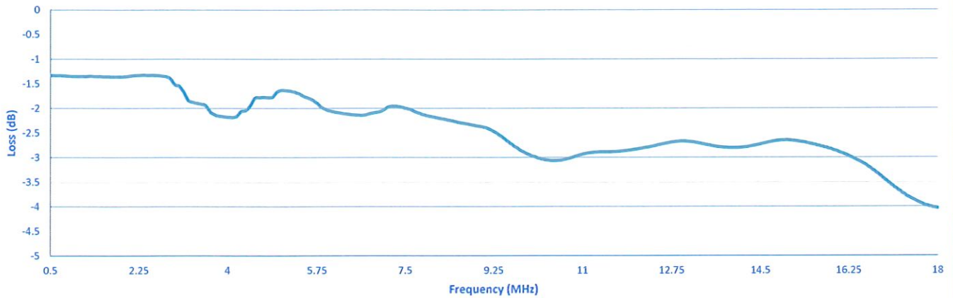
Insertion Loss
