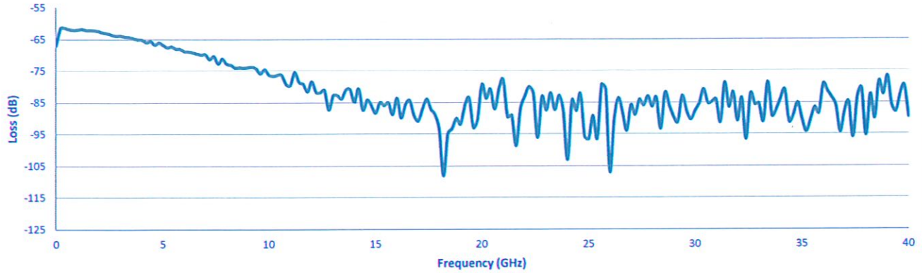
Isolation
