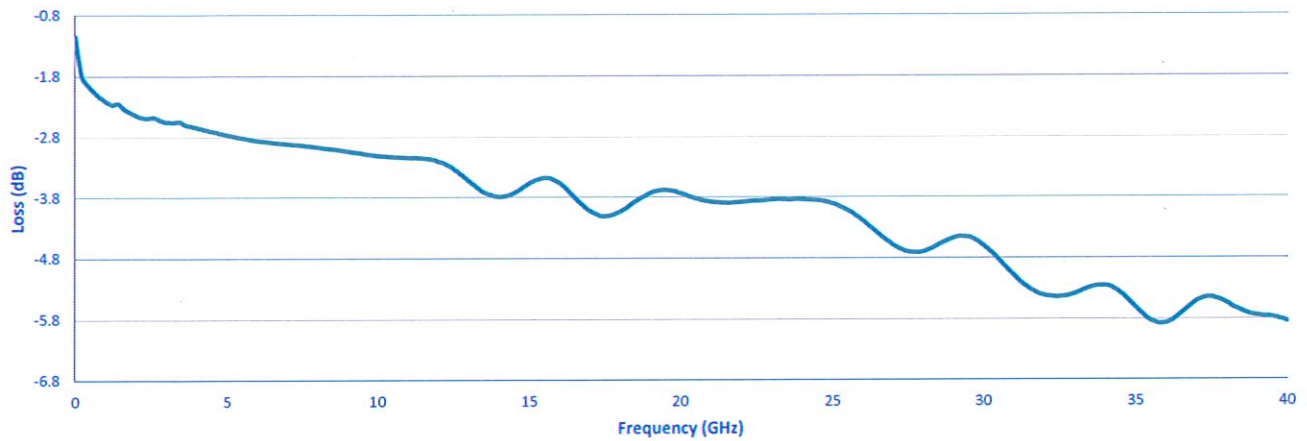
Insertion Loss
