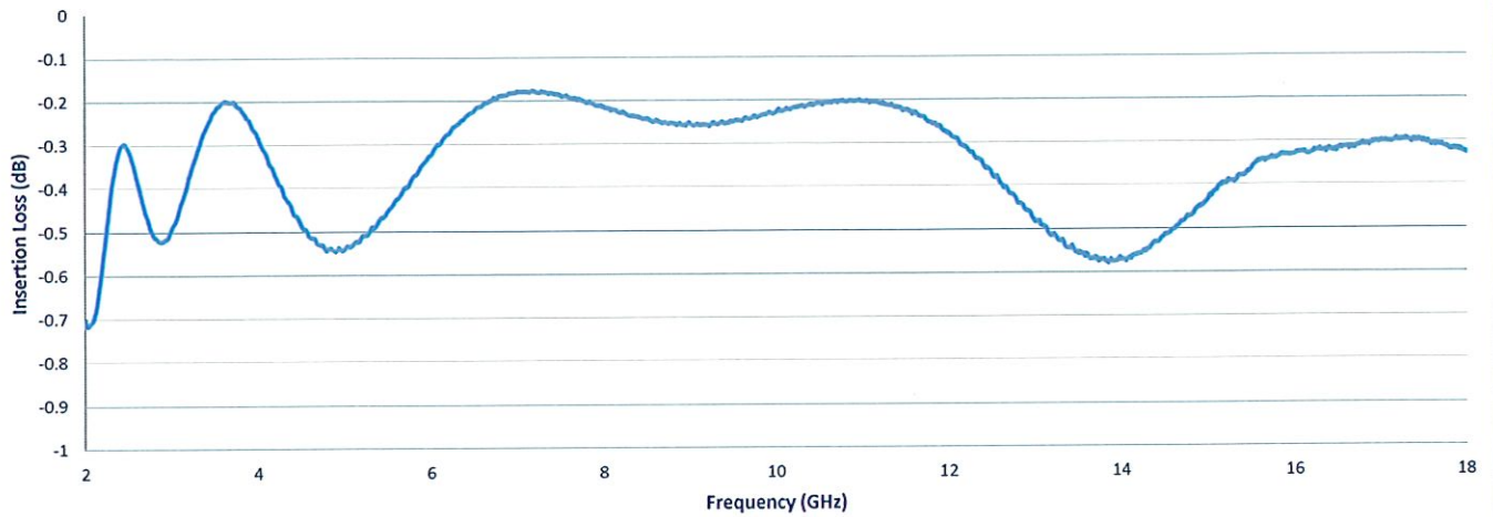
Insertion Loss vs Frequency (@PassBand)
