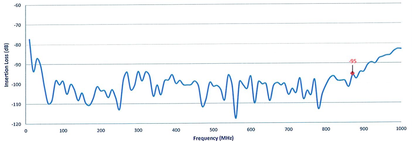
Rejection vs Frequency
