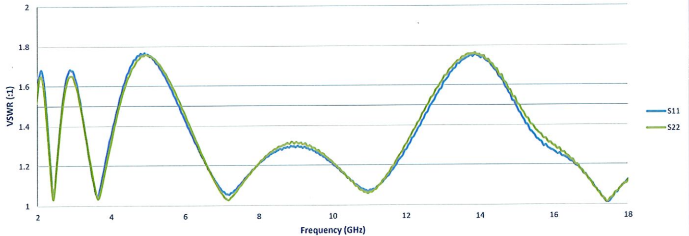
VSWR vs Frequency (@PassBand)
