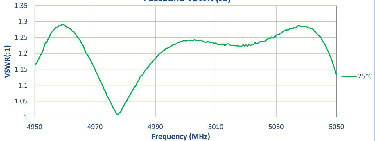
Passband VSWR (J2)
