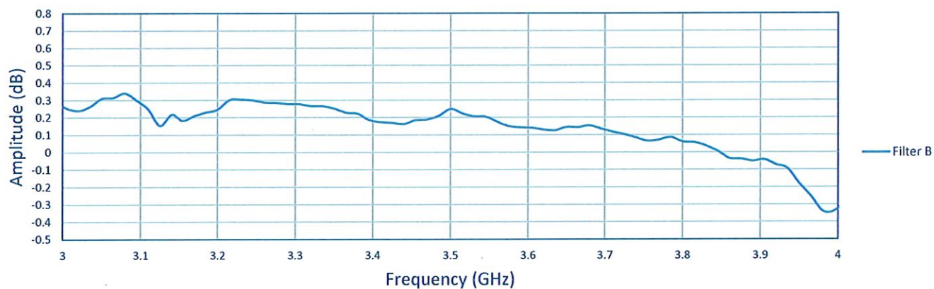
3 - 4 GHz Filter Ripple
