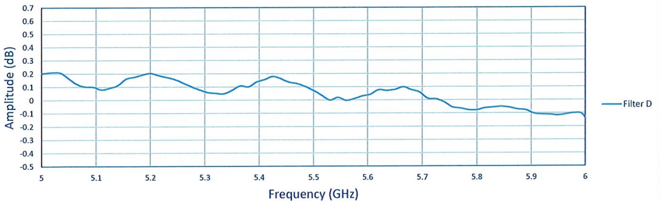
5 - 6 GHz Filter Ripple
