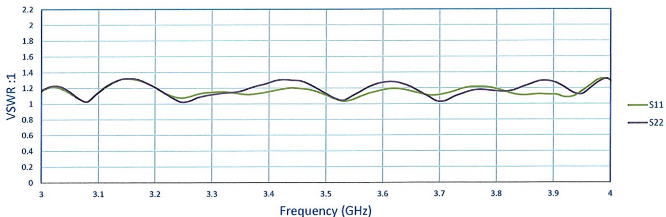
VSWR 3 - 4 GHz Filter
