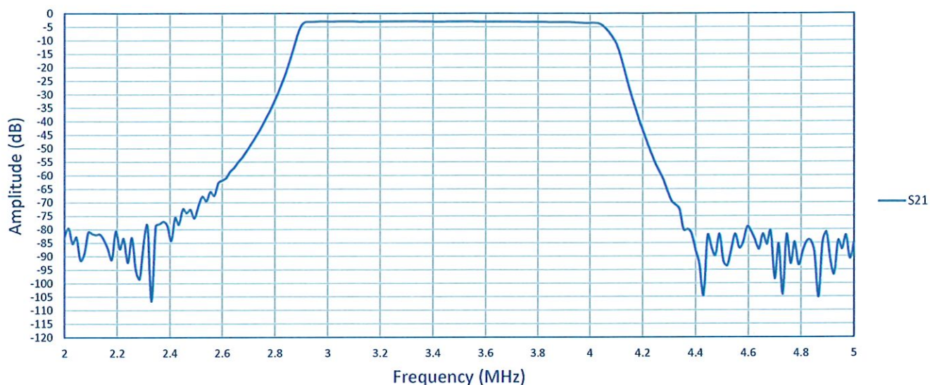
3 - 4 GHz Filter
