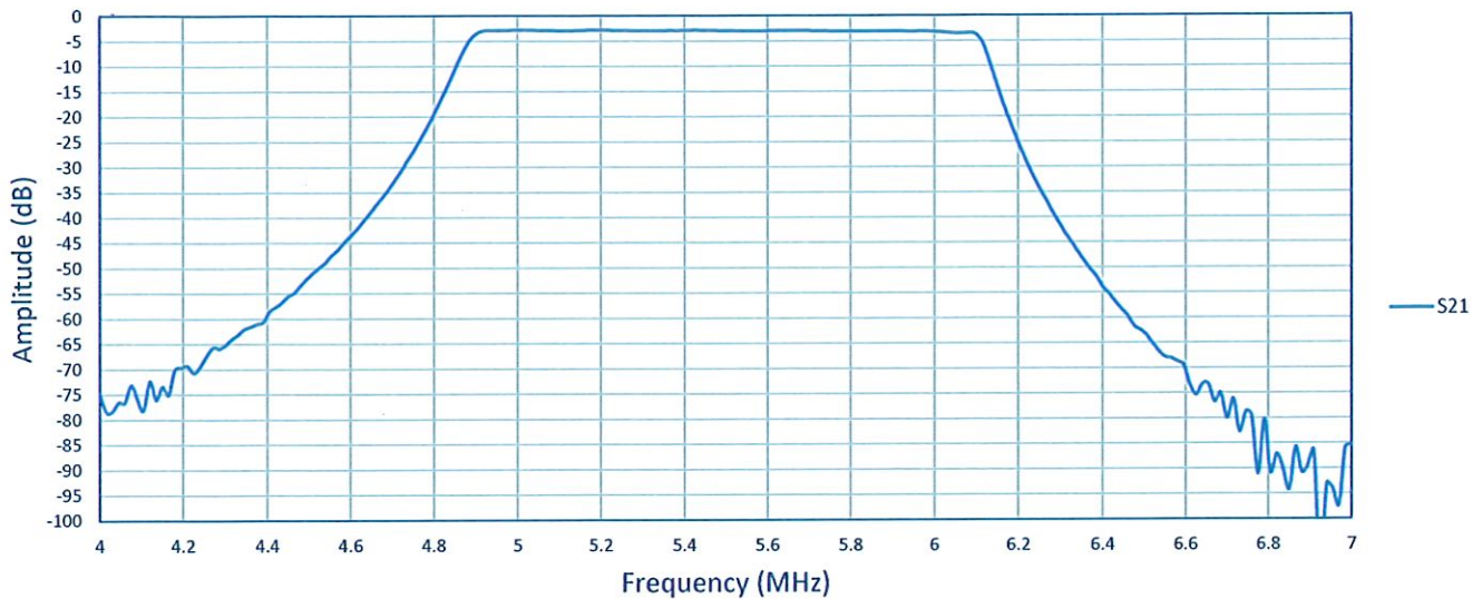
5 - 6 GHz Filter
