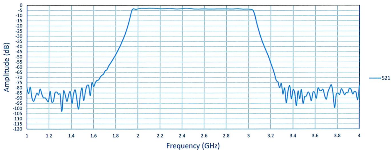
2 - 3 GHz Filter
