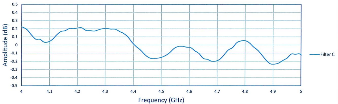
4 - 5 GHz Filter Ripple
