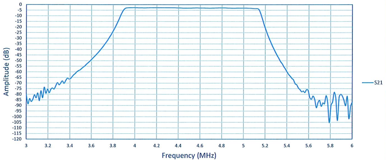
4 - 5 GHz Filter
