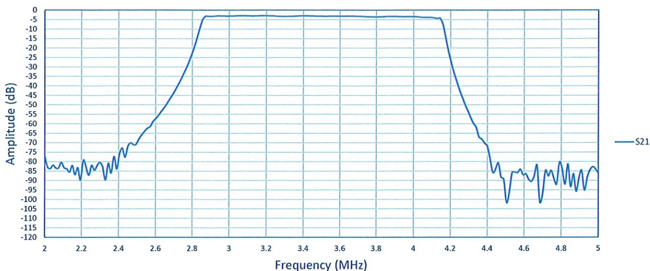
3 - 4 GHz Filter
