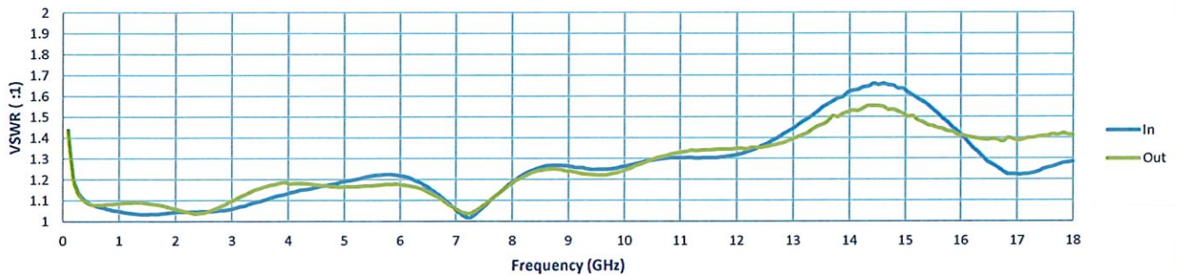
VSWR @ -20 dBm
